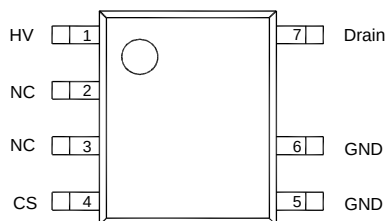
SOP-7
