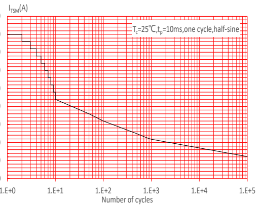
FIG.6: Non-repetitive surge peak on-state current for a sinusoidal pulse with width t_p < 10ms , and corresponding value of I^2t ( di/dt < 50A/μs )
